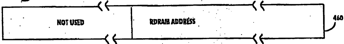
Fig. 7D SP MEMORY DMA ADDRESS (R/W)
